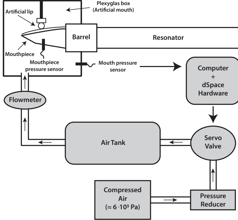
FIGURE 5.3 – Principle of the Pressure Controlled Artificial Mouth (PCAM).
