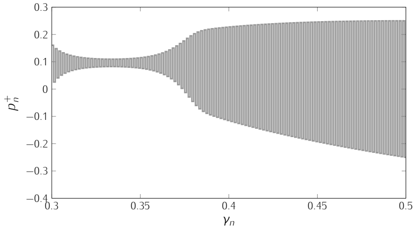
FIGURE 2.7 – Representation of the series p_n^+ as a function of \gamma_n for \zeta = 0.5, \epsilon = 10^{-3}, \gamma_0 = 0.3 and p_0^+ = G(0, \gamma_0) .
