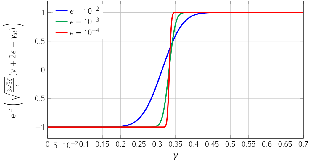
FIGURE 4.13 – Graphical representation of the function \text{erf}\left(\sqrt{\frac{3\sqrt{3}\zeta}{\epsilon}}(\gamma + 2\epsilon - \gamma_{st})\right) as a function of \gamma as for \zeta = 0.5 and for three different values of the slope \epsilon .
